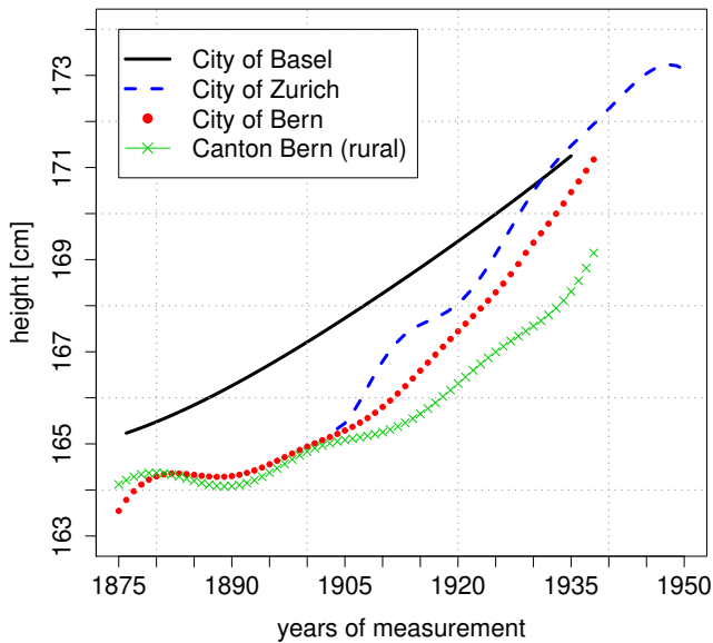
Figure 2: Secular trends (yearly averages) of the canton Bern (1875–1938), Basel (1875–1935), and Zurich (1904–1950); all series were smoothed by local polynomial regression.
