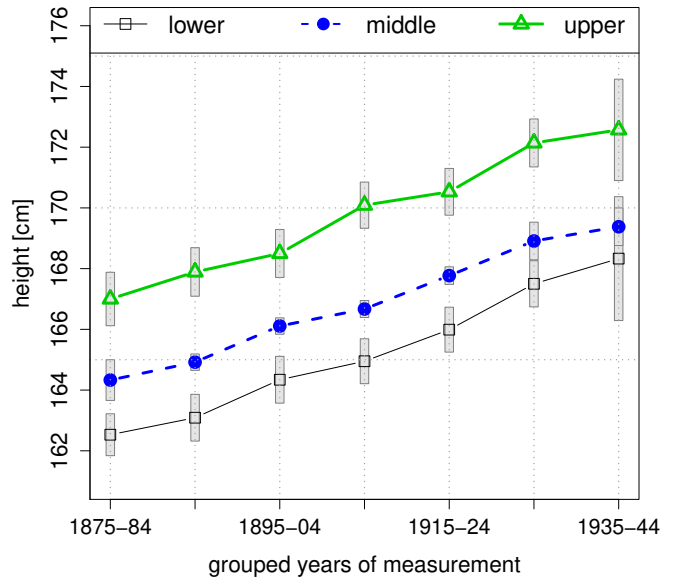
Figure 4: Class-specific time trajectories of average height (1875–1935). The data are predictions from the models in Table 1. The bars denote 95 % confidence intervals.
