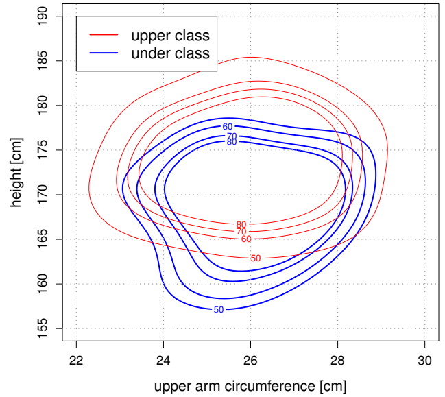
Figure 10: Contour plot of the bivariate kernel density estimates of height versus upper arm circumference (Zurich 1933 conscription data; N=1795 ; kernel: Epanechnikov; bandwidth selection: smoothed cross-validation with bandwidth matrix constrained to be diagonal).
