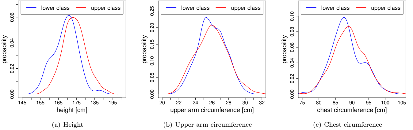
Figure 6: Class-specific kernel density estimates of height, chest and upper arm circumference (Zurich 1933 conscription data; N = 1795 ; Epanechnikov kernel).
