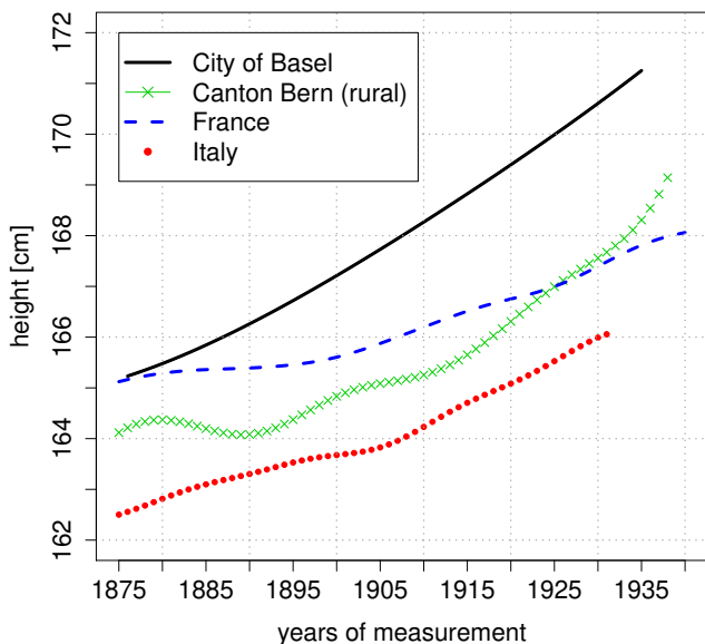
Figure 3: Secular trends (yearly average) of Switzerland, France (Van Meerten, 1990), and Italy (Federico, 2003); all series were smoothed by local polynomial regression.
