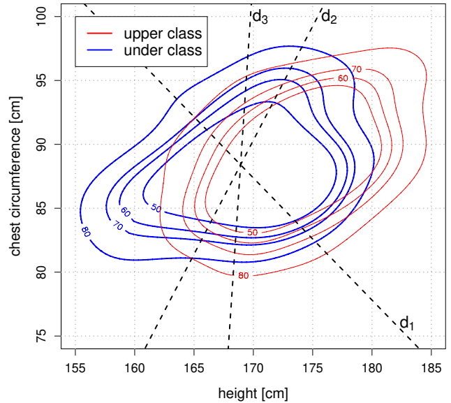
Figure 7: Contour plot of the bivariate kernel density estimates of height versus chest circumference (Zurich 1933 conscription data; N=1795 ; kernel: Epanechnikov; bandwidth selection: unconstrained smoothed cross-validation).
