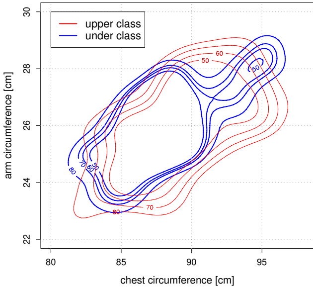
Figure 9: Contour plot of the bivariate kernel density estimates of chest versus upper arm circumference (Zurich 1933 conscription data; N=1795 ; kernel: Epanechnikov; bandwidth selection: unconstrained smoothed cross-validation).
