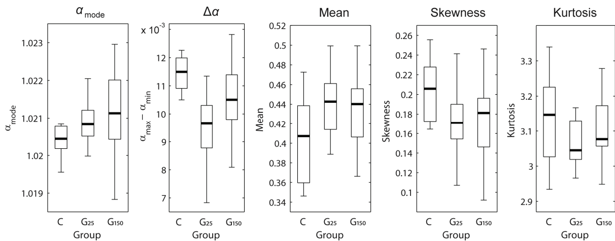
Figure 2. Boxplots of the determined values of multifractal parameters ( \alpha_{mode} , \Delta\alpha ) and classical parameters (mean, skewness and kurtosis).
