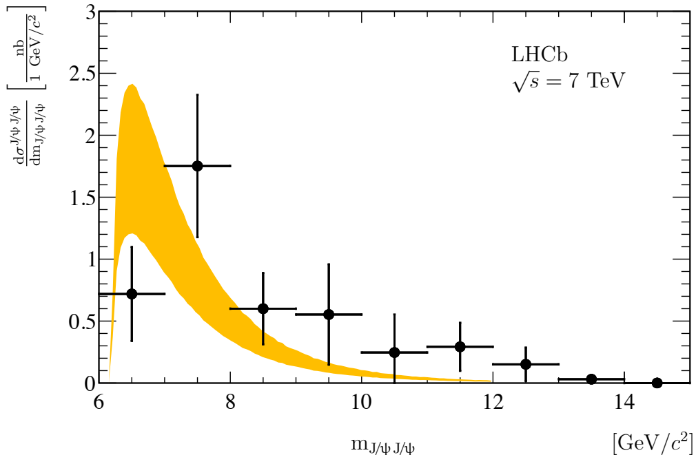
Figure 2: Differential production cross-section for J/\psi pairs as a function of the invariant mass of the J/\psi J/\psi system. The points correspond to the data. Only statistical uncertainties are included in the error bars. The shaded area corresponds to prediction by the model described in Ref. [20].
