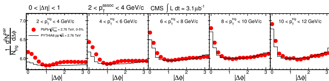
Figure 2. Short-range ( |\Delta\eta| < 1 ) per-trigger-particle associated yields of charged hadrons as a function of |\Delta\phi| from the 0-5% most central PbPb collisions at \sqrt{s_{NN}} = 2.76 TeV, requiring 2 < p_T^{\text{assoc}} < 4 GeV/c, for five different intervals of p_T^{\text{trig}} . The PYTHIA8 pp MC results (solid histograms) are also shown, shifted up by a constant value to match the PbPb data at \Delta\phi = 1 for ease of comparison. The error bars are statistical only and are too small to be visible in most of the panels. The systematic uncertainty of 7.6% for all data points is not shown in the plots.
