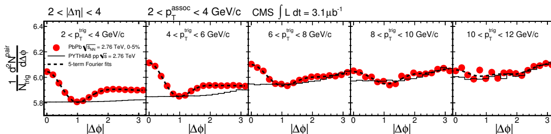
Figure 3. Long-range ( 2 < |\Delta\eta| < 4 ) per-trigger-particle associated yields of charged hadrons as a function of |\Delta\phi| under the same conditions as in figure 2. The systematic uncertainty of 7.3% for all data points is not shown in the plots. Dashed lines show the fits by the first five terms in the Fourier series, as discussed in section 3.3.
