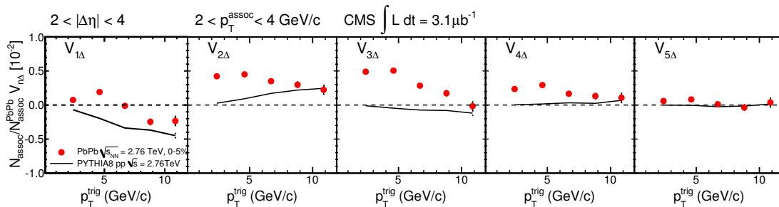
Figure 6. Fourier coefficients, V_{1\Delta} , V_{2\Delta} , V_{3\Delta} , V_{4\Delta} , and V_{5\Delta} , extracted as functions of p_T^{\text{trig}} for 2 < p_T^{\text{assoc}} < 4 \text{ GeV}/c for the 0-5% most central PbPb collisions at \sqrt{s_{\text{NN}}} = 2.76 \text{ TeV} . The error bars represent statistical uncertainties only. The solid lines show the predictions from the PYTHIA8 simulation of pp collisions at \sqrt{s} = 2.76 \text{ TeV} .
