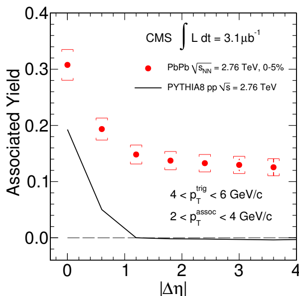
Figure 4. Integrated near-side ( |\Delta\phi| < \Delta\phi_{\text{ZYAM}} ) associated yield for 4 < p_{\text{T}}^{\text{trig}} < 6 \text{ GeV}/c and 2 < p_{\text{T}}^{\text{assoc}} < 4 \text{ GeV}/c , above the minimum level found by the ZYAM procedure, as a function of |\Delta\eta| for the 0-5% most central PbPb collisions at \sqrt{s_{\text{NN}}} = 2.76 \text{ TeV} . The error bars correspond to statistical uncertainties, while the brackets denote the systematic uncertainties. The solid line shows the prediction from the PYTHIA8 simulation of pp collisions at \sqrt{s} = 2.76 \text{ TeV} .
