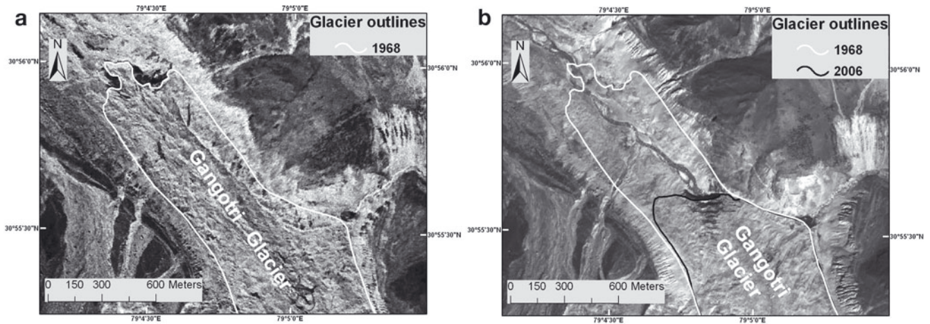
Fig. 9. Frontal area images of Gangotri Glacier. (a) Corona image (27 September 1968) with same-year glacier outline, (b) Cartosat-1 image (11 October 2006) with glacier outline of 1968 and 2006.
