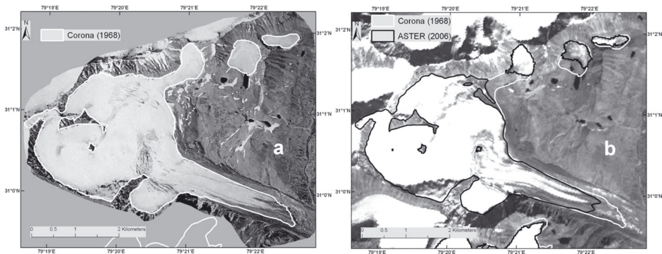
Fig. 3. Satellite images of Tara Bamak Glacier, Saraswati/Alaknanda basin (see Fig. 1 for location). (a) Rectified subset of Corona image (27 September 1968) based on spline method with similar-year glacier outline. (b) ASTER image (11 October 2006) with ASTER and Corona glacier outlines.
