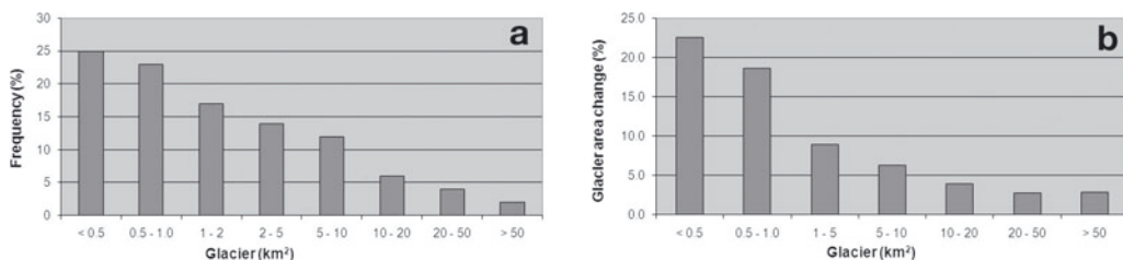
Fig. 5. (a) Area frequency distribution of glaciers for both the Saraswati/Alaknanda and upper Bhagirathi basins derived from analysis of ASTER (11 October 2006) image. (b) Glacier area change and area measurements (%) based on Corona (27 September 1968) and ASTER (11 October 2006) images in both the Saraswati/Alaknanda and upper Bhagirathi basins.
