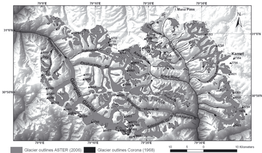
Fig. 6. Glacier change in the Garhwal Himalaya from 1968 to 2006.
