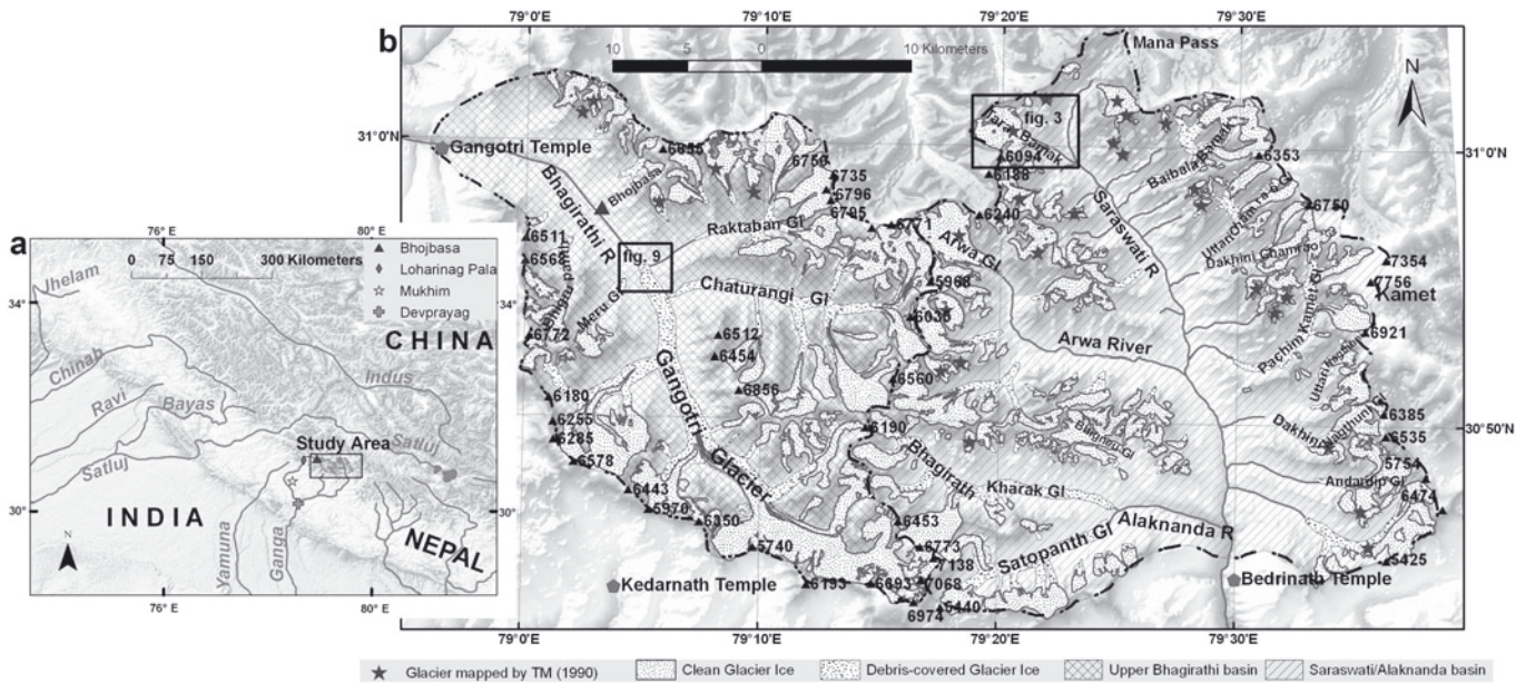
Fig. 1. (a) Location of study area in the Himalaya with major river systems of the Indian subcontinent. (b) Glacier coverage in the upper Bhagirathi and Saraswati/Alaknanda basins, based on ASTER (11 October 2006) imagery; stars represent glaciers mapped from Landsat Thematic Mapper (TM) (15 November 1990)
