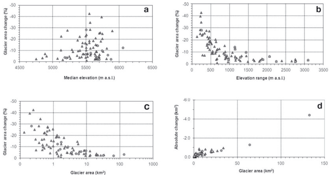
Fig. 7. Scatter plots of (a) median elevation vs glacier area change (%), (b) elevation range vs glacier area change (%), (c) glacier area ( \text{km}^2 ) vs glacier area change (%) and (d) glacier area ( \text{km}^2 ) vs absolute glacier area change ( \text{km}^2 ). Triangles are for the Saraswati/Alaknanda basin and circles are for the Bhagirathi basin. Glacier area change (%) derived from analysis of Corona (27 September 1968) and ASTER (11 October 2006) images.
