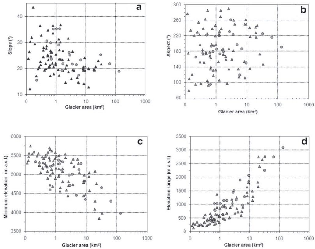
Fig. 4. Scatter plots of (a) glacier area vs slope, (b) glacier area vs aspect, (c) glacier area vs minimum elevation and (d) glacier area vs elevation range. Triangles are for the Saraswati/Alaknanda basin and circles are for the Bhagirathi basin. Glacier area and inventory data derived from ASTER (11 October 2006) image and DEM.
