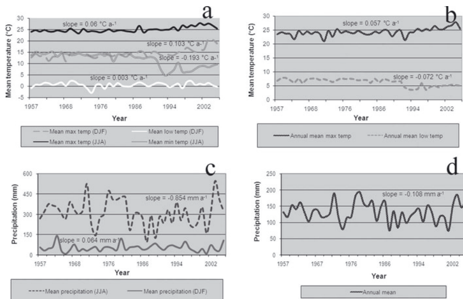
Fig. 8. Climate parameters for Mukhim station: (a) mean T_{\text{MAX}} and T_{\text{MIN}} for DJF and JJA from 1957 to 2005; (b) mean annual T_{\text{MAX}} and T_{\text{MIN}} ; (c) mean minimum and maximum precipitation for DJF and JJA; and (d) annual mean precipitation. DJF: December, January, February; JJA: June, July, August.
