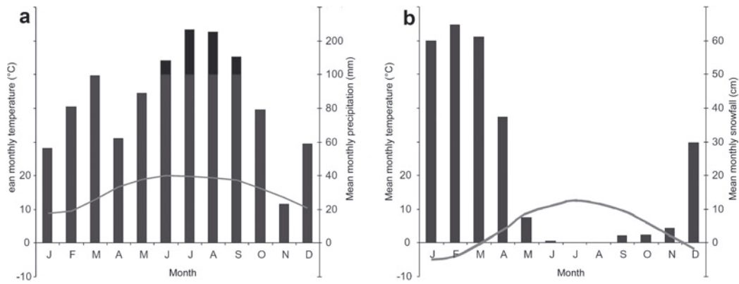
Fig. 2. Climate data for (a) Mukhim (~1900 m a.s.l.; MAAT 15.4°C, annual precipitation 1648 mm, 1971–2000) and (b) Bhojbasa stations (~3780 m a.s.l., 4.4°C; 2001–09) (see Fig. 1 for location). Data sources: Indian Meteorological Department (IMD) and Snow and Avalanche Study Establishment (SASE).
