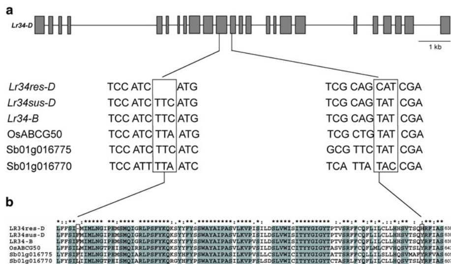
Fig. 1 Resistant and susceptible Lr34 haplotypes a Gene structure of Lr34 . Grey boxes indicate exons; introns are shown as adjoining lines. The two critical codons in exons 11 and 12 that differ between Lr34 alleles of resistant and susceptible wheat cultivars are framed. b Alignment showing residues 541–639 of the wheat LR34 protein and the corresponding regions from the homoeologous LR34-B protein as well as the orthologous proteins from rice and sorghum. The two critical residues that differ between LR34res-D and LR34sus-D are framed. Residues marked in grey are conserved in
