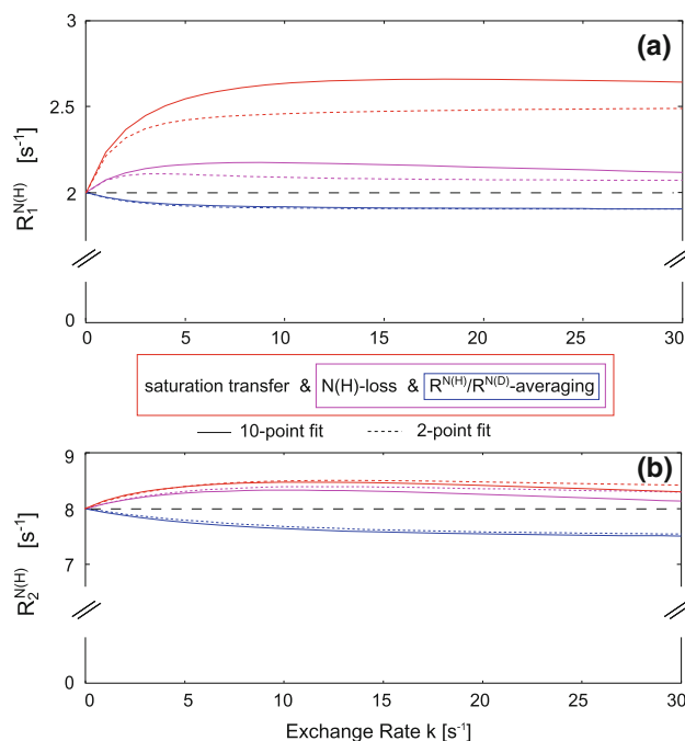
Fig. 3 Apparent R_1 (a) and R_2 rates (b) as a function of the exchange rate k , calculated with (red lines) and without (purple lines) \tau -dependent water saturation. Alternatively, curves for experiments just starting with equilibrium ^{15}\text{N} magnetization are additionally shown (blue lines). The solid lines are obtained from least-squares fits of frequently sampled data ( R_1 - \tau 's: 0.005, 0.01, 0.02, 0.04, 0.08, 0.16, 0.32, 0.64, 1.28, and 2.56 s; R_2 - \tau 's: 0.014, 0.028, 0.042, 0.056, 0.07, 0.098, 0.14, 0.21, 0.28 and 0.42 s) whereas the dashed lines are obtained by the two-point sampling strategy ( R_1 - \tau 's: 0 and 0.65 s; R_2 - \tau 's: 0 and 0.16 s). The black dashed lines describe the theoretical curves using rates of 2 \text{ s}^{-1} ( R_1 ) or 8 \text{ s}^{-1} ( R_2 ). 10 % deuterated solvent ( x = 0.1 ) was assumed in all simulations, and the relaxation rates of deuterated species were assumed to be 1 \text{ s}^{-1} ( R_1^{N(D)} ) or 2.9 \text{ s}^{-1} ( R_2^{N(D)} ) respectively. The effect of water saturation was calculated using p_{(\tau)} = 0.75 e^{-1.7\tau} for the R_1 - and p_{(\tau)} = 0.7 + 0.24\tau - 2.7\tau^2 for the R_2 -experiment, respectively. (Color figure online)
