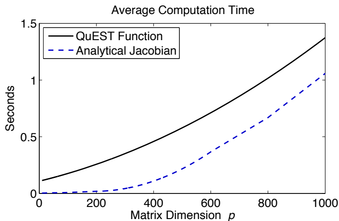
Figure 1: Average computation time for the QuEST function and its analytical Jacobian. The setup is the same as in Figure 2 below. The QuEST function and its analytical Jacobian are programmed in Matlab. The computer is a 2.4 GHz Quad-Core Intel Xeon desktop Mac.
