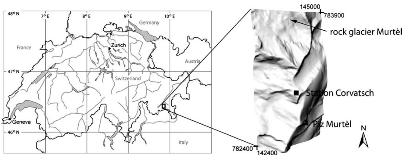
Figure 1 Location of the study site and topography of the test area in a 3D visualization
