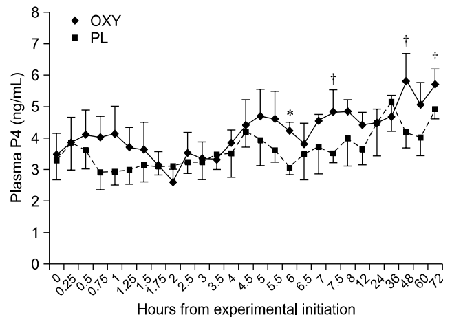
Fig. 4. Levels of plasma progesterone (P4 in \text{ng/mL} ) 72 h after OXY ( p = 0.07 ) or PL ( p = 0.14 ) infusion in Holstein-Friesian cows. Data represent mean \pm SE. * p = 0.01 , † p = 0.08 .
