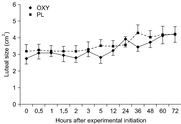
Fig. 1. Luteal size ( \text{cm}^2 ) 72 h after oxytocin (OXY, p = 0.02 ) or placebo (PL, p = 0.001 ) infusion in Holstein-Friesian cows. Data represent mean \pm SE.
