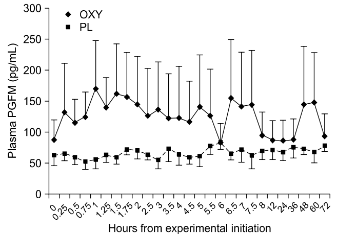
Fig. 3. Levels of plasma prostaglandin metabolites (PGFM, \text{pg/mL} ) 72 h after OXY or PL infusion in Holstein-Friesian cows. Data represent mean \pm SE.
