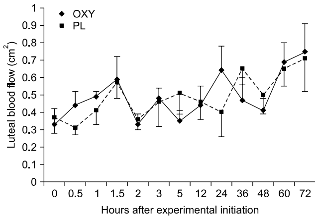
Fig. 2. Luteal blood flow ( \text{cm}^2 ) 72 h after OXY or PL infusion in Holstein-Friesian cows. Data represent mean \pm SE.
