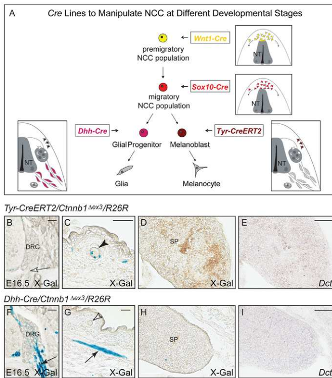
Fig. 7. Ectopic melanoblasts are derived from migratory neural crest cells rather than from melanoblasts or glial progenitors.
