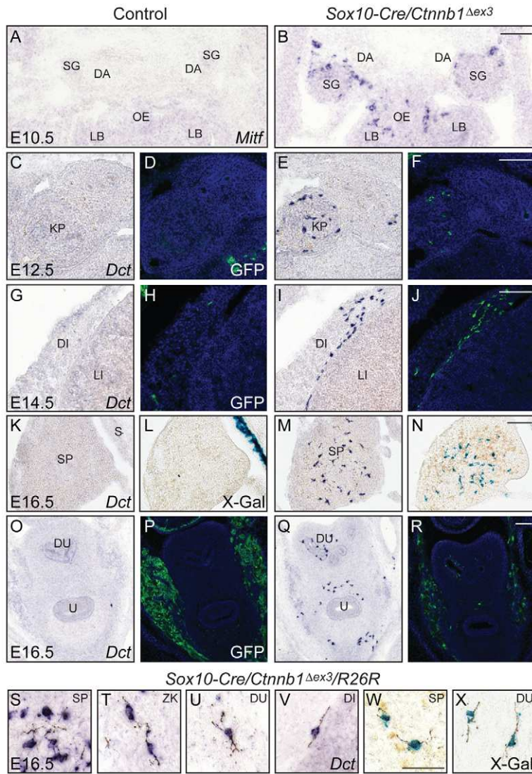
Fig. 6. Formation of ectopic melanoblasts at various locations in Sox10-Cre/Ctnnb1 Δex3 embryos. Ectopic Dct - and Mitf -positive melanoblasts are detected by in situ hybridization on transverse sections using Mitf (A,B) and Dct (C-V) riboprobes. The neural crest origin of the Dct - and Mitf -positive melanoblasts is illustrated by anti-GFP or X-Gal staining using mouse embryos carrying the Z/EG or R26R reporter lines, respectively. (A-R) The following examples of organs populated by Dct - and Mitf -positive melanoblasts in Sox10-Cre/Ctnnb1 Δex3 embryos are shown: tissue surrounding the sympathetic ganglia (SG) and the lung buds (LB) at E10.5 (A,B); the kidney primordium (KP, C-F) at E12.5; the diaphragm (DI, G-J) at E14.5; the spleen (SP, K-N) at E16.5; the urogenital tract, around the urethra (U) and the reproductive ducts (DU, O-R) at E16.5. (S-V) Pigmentation of Dct -positive ectopic cells in Sox10-Cre/Ctnnb1 Δex3 embryos demonstrates their melanocyte identity. Examples of pigmented cells are shown in the spleen (S), in the ganglion of Zuckerkandl (ZK, T), around the reproductive ducts (U) and in the diaphragm (V). (W,X) X-Gal staining shows recombination in these pigmented melanocytes; cells in the spleen (W) and around the reproductive ducts (X) are shown as examples. Note the absence of neural crest-derived cells in all locations of ectopic Dct -positive cells in control embryos, as revealed by X-Gal and anti-GFP staining (D,H,L,P). DA, dorsal aorta; OE, oesophagus; LI, liver; S, stomach. Scale bars: 100 μm in A-R; 50 μm in S-X.
