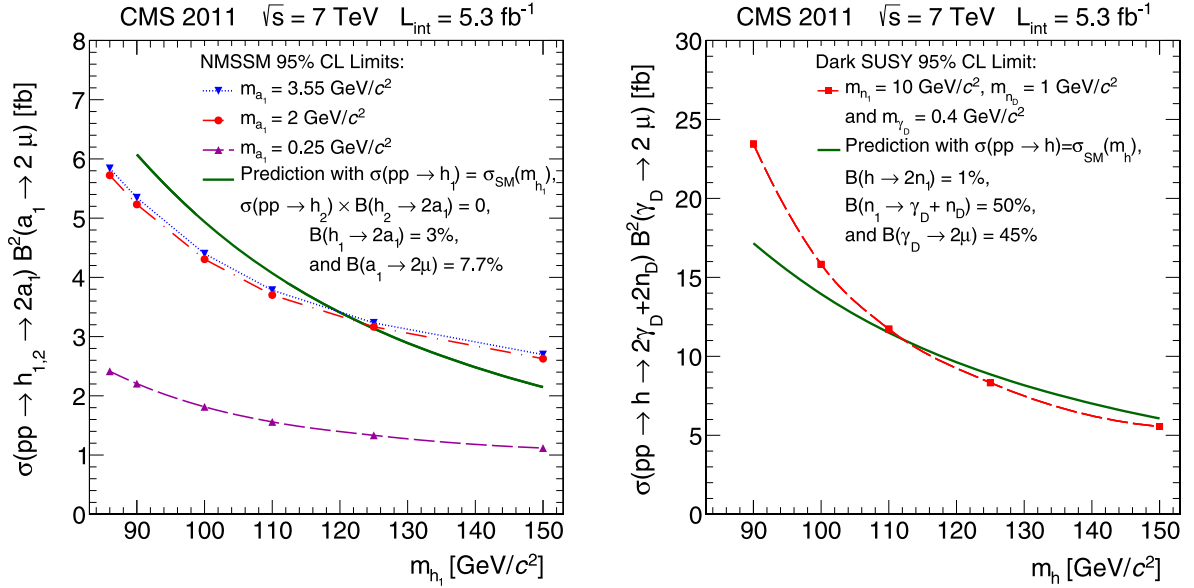
Fig. 2. Left: The 95% CL upper limits as functions of m_{h_1} , for the NMSSM case, on \sigma(pp \rightarrow h_{1,2} \rightarrow 2a_1) \times B^2(a_1 \rightarrow 2\mu) with m_{a_1} = 0.25 \text{ GeV}/c^2 (dashed curve), m_{a_1} = 2 \text{ GeV}/c^2 (dash-dotted curve) and m_{a_1} = 3.55 \text{ GeV}/c^2 (dotted curve). As an illustration, the limits are compared to the predicted rate (solid curve) obtained using a simplified scenario with \sigma(pp \rightarrow h_1) = \sigma_{\text{SM}}(m_{h_1}) [65], \sigma(pp \rightarrow h_2) \times B(h_2 \rightarrow 2a_1) = 0 , B(h_1 \rightarrow 2a_1) = 3\% , and B(a_1 \rightarrow 2\mu) = 7.7\% . The chosen B(a_1 \rightarrow 2\mu) is taken from [28] for m_{a_1} = 2 \text{ GeV}/c^2 and NMSSM parameter \tan\beta = 20 . Right: The 95% CL upper limit as a function of m_{h_1} , for the dark-SUSY case, on \sigma(pp \rightarrow h \rightarrow 2\eta_1 \rightarrow 2\eta_D + 2\gamma_D) \times B^2(\gamma_D \rightarrow 2\mu) with m_{h_1} = 10 \text{ GeV}/c^2 , m_{h_D} = 1 \text{ GeV}/c^2 and m_{\gamma_D} = 0.4 \text{ GeV}/c^2 (dashed curve). As an illustration, the limit is compared to the predicted rate (solid curve) obtained using a simplified scenario with SM Higgs boson production cross section \sigma(pp \rightarrow h) = \sigma_{\text{SM}}(m_h) [65], B(h \rightarrow 2\eta_1) = 1\% , B(\eta_1 \rightarrow \eta_D + \gamma_D) = 50\% , and B(\gamma_D \rightarrow 2\mu) = 45\% . The chosen B(\gamma_D \rightarrow 2\mu) is taken from [31] for m_{\gamma_D} = 0.4 \text{ GeV}/c^2 .
