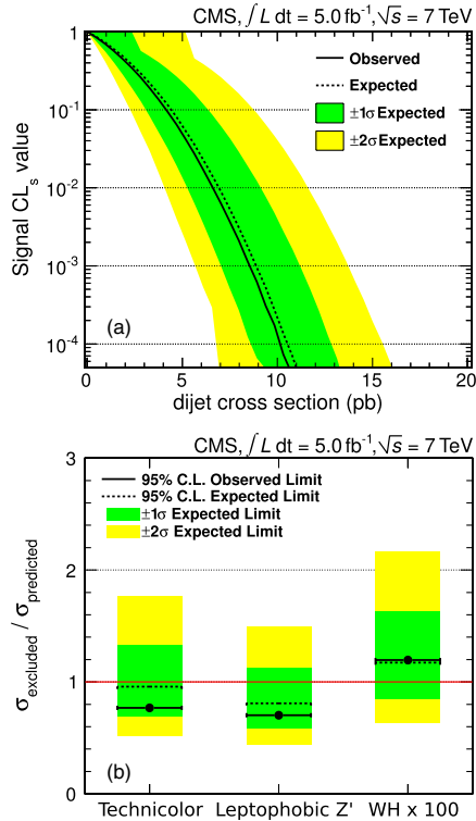
FIG. 2 (color online). (a) The observed and expected values of the CL_s statistic for a generic Gaussian signal hypothesis with M = 150 \text{ GeV} and \sigma_{jj} = 15 \text{ GeV} , as a function of the dijet signal cross section. (b) Observed and expected 95% C.L. upper limits, with one- and two-sigma error bands, on the cross section divided by the expected values for various signal models. The limits are calculated using the CL_s method. A value of the excluded cross section over the predicted cross section of less than one indicates that the model is excluded at 95% C.L. Table III lists the cross sections for these models.
