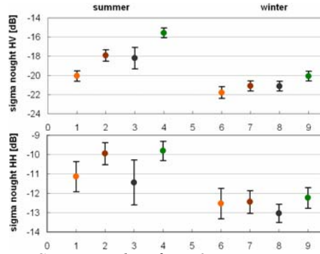
Figure 4. Signature plot of HV & HH intensity. 1 & 6 = recent clear-cut, 2 & 7 = former clear-cut, 3 & 8 = fire scar, 4 & 9 = forest. Error bars flag std. deviation
