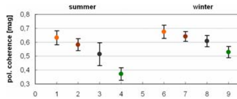
Figure 6. Signature plot of |\rho_{HHVV}|
