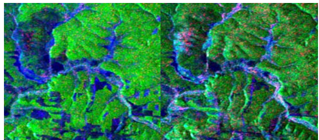
Figure 9. Freeman decomposition ( P_v/P_d/P_s ). Left: summer, Right: winter
