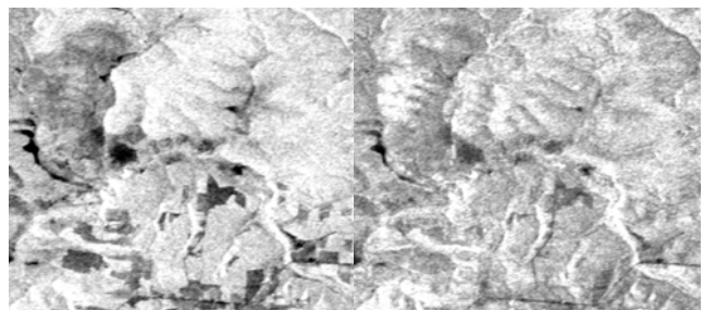
Figure 11. Krogager decomposition coefficient |k_d|^2 (dipole component). Left: summer, Right: winter
