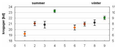
Figure 12. Signature plot of |kd|^2 (diplane component)
