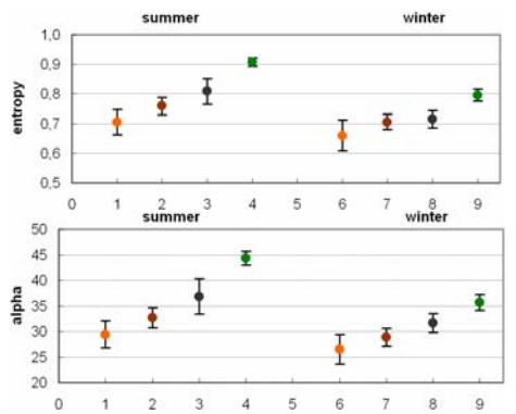
Figure 8. Signature plots of entropy & alpha
