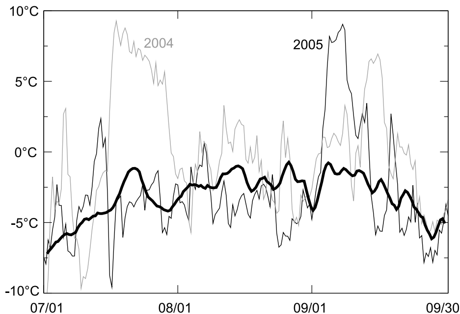
Fig. 3. July through September (JAS) temperature record at 3000 meters (approximately at the Mount Steller summit) from the Yakutat radiosonde, showing the large positive temperature anomaly in 2004 and 2005. The bold curve represents the 1994–2007 JAS average. Values are plotted with date (month/day) on the x-axis and temperature on the y-axis.
