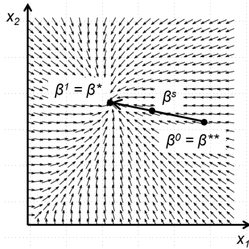
Figure 2. Illustration of the uniqueness proof
