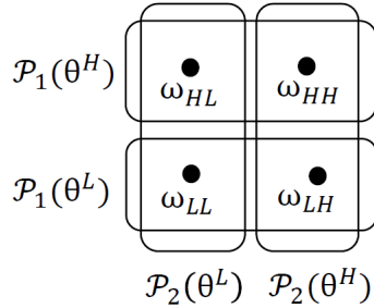
Figure 1. Information structure in Example 1
