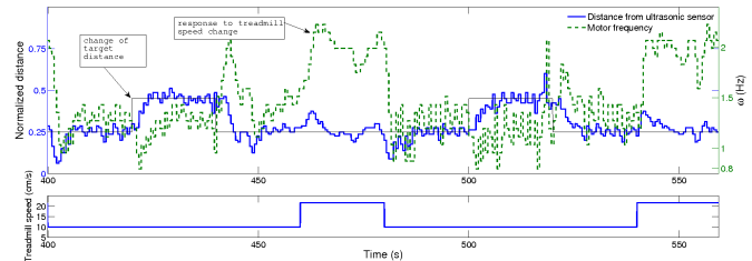
Fig. 2 Speed adaptation performance. The top graph shows the target (target distance - black line) tracking performance by the robot (actual distance measured by sensor in blue; distance had a range 10-90 cm and was normalized). When the target moves, the robot needs to respond with an appropriate change in frequency (green dotted line). The same applies when the treadmill speed (bottom graph) changes.
