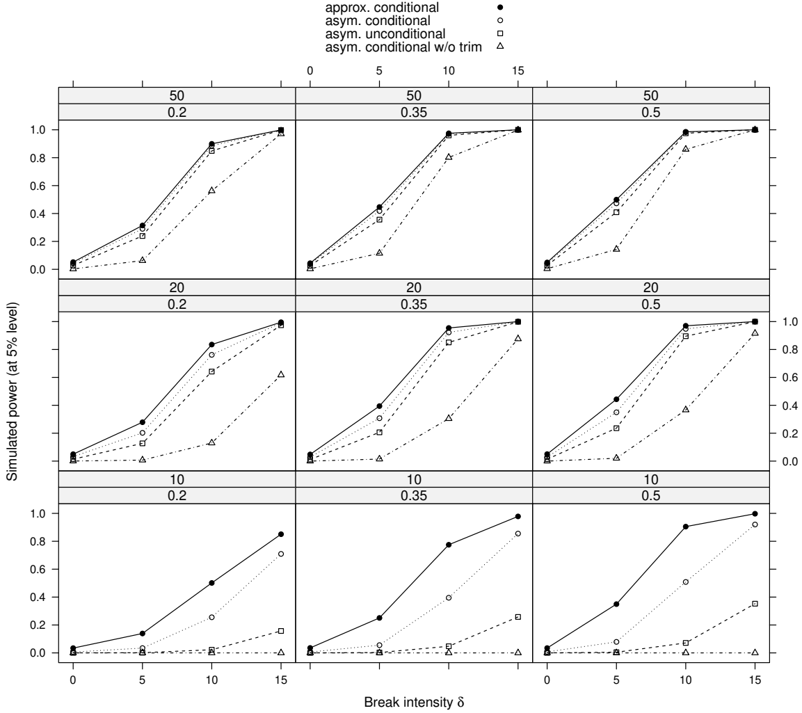
Figure 1: Simulated power of the \text{supLM} tests using reference distributions: approximated conditional \mathcal{D}_{\sigma|Y} (solid, solid circles), asymptotic conditional \mathcal{D}_{\infty|Y} (dotted, hollow circles), asymptotic unconditional \mathcal{D}_{\infty} (dashed, hollow squares), asymptotic conditional without trimming \mathcal{D}_{\infty|Y}^0 (dash-dotted, hollow triangles).
