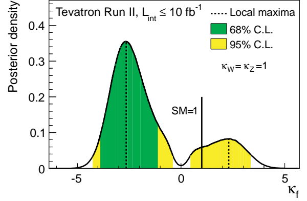
FIG. 19: (color online). Posterior probability density for \kappa_f from the combination of Tevatron searches for a SM-like Higgs boson with m_H = 125 \text{ GeV}/c^2 . The couplings of the Higgs boson to the W^\pm and Z bosons are assumed to be as predicted by the SM. The values that maximize the local posterior probability densities are shown with dashed lines, and the 68% and 95% C.L. intervals are indicated with the dark- and light-shaded regions, respectively. The predicted SM value of \kappa_f is indicated by the solid vertical line.
